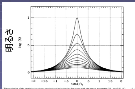
Time variation of the amplification due to gravitational microlensing for events with the impact parameter u , equal 0.1, 0.2, ..., 1.1, 1.2
