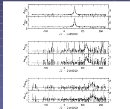
FIG. 1.—The light curves of the three candidate microlensing events. The solid lines show the best fit microlensing curves, with the parameters shown in Table 1. Units as in Fig. 3.
