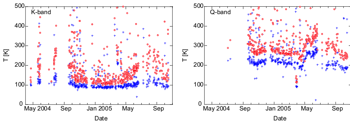
Figure 12: The receiver noise temperature ( blue crosses ) and the system noise temperature ( red open circles ) at the zenith in the K band and the Q band with the Mizusawa antenna.
