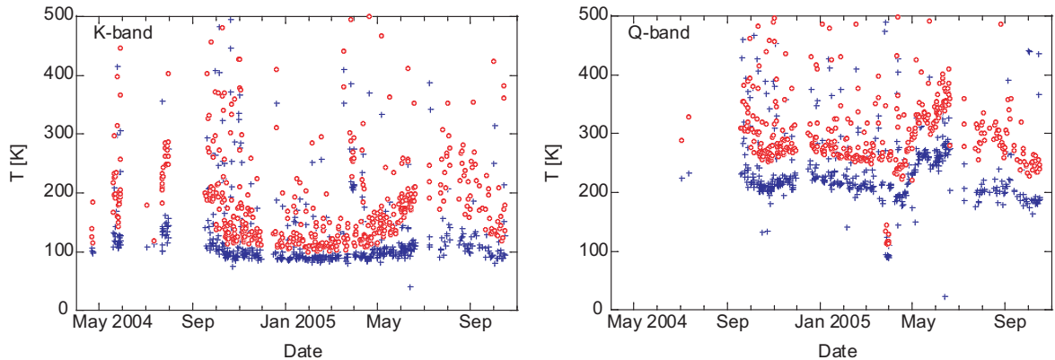
Figure 14: The receiver noise temperature ( blue crosses ) and the system noise temperature ( red open circles ) at the zenith in the K band and the Q band with the Mizusawa antenna.
