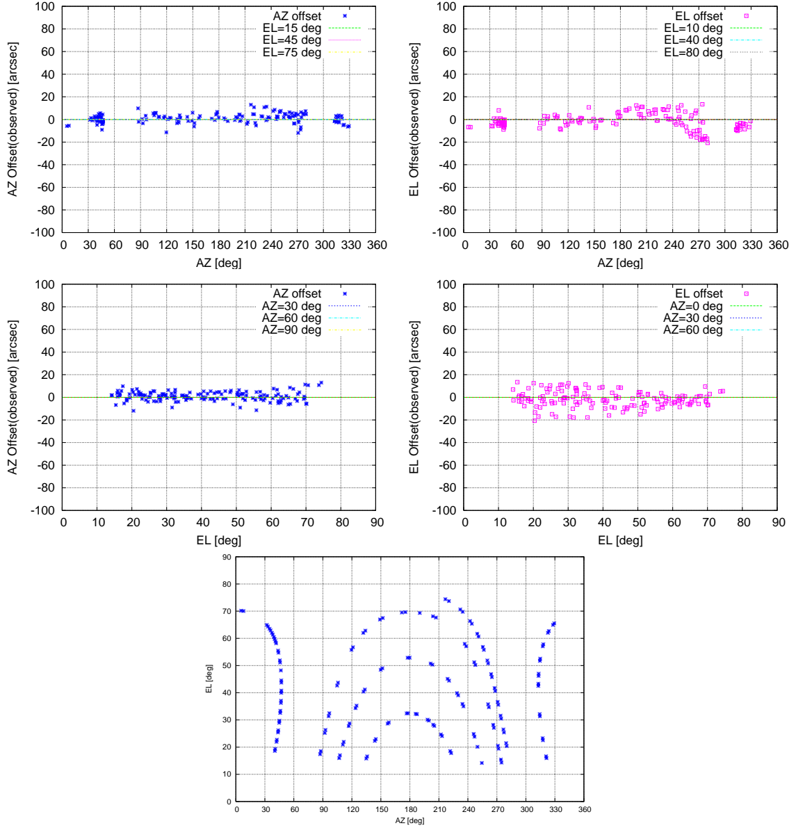
Figure 7: Examples of pointing residuals for the Iriki antenna in the Q band (43 GHz). Top and middle panels show relations of the azimuth and elevation, respectively, with the pointing residuals in azimuth ( left ) and elevation ( right ). Bottom panel shows positions on celestial sphere of the objects which were observed in the pointing measurement.
