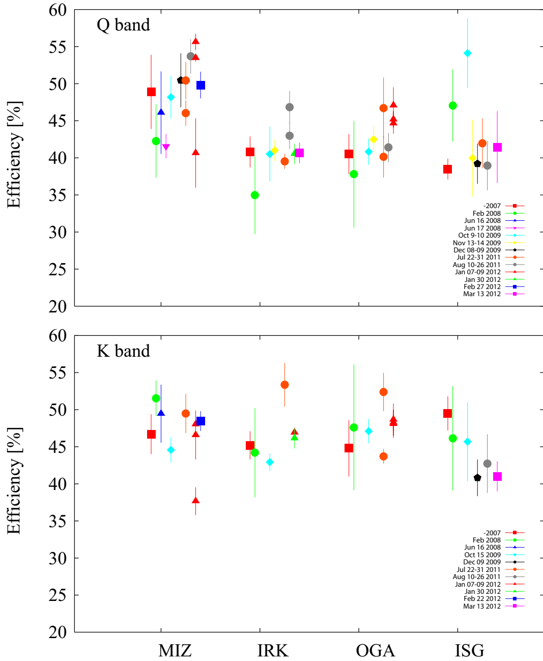
Figure 3: History of the aperture efficiency measurements for the VERA antennas.
