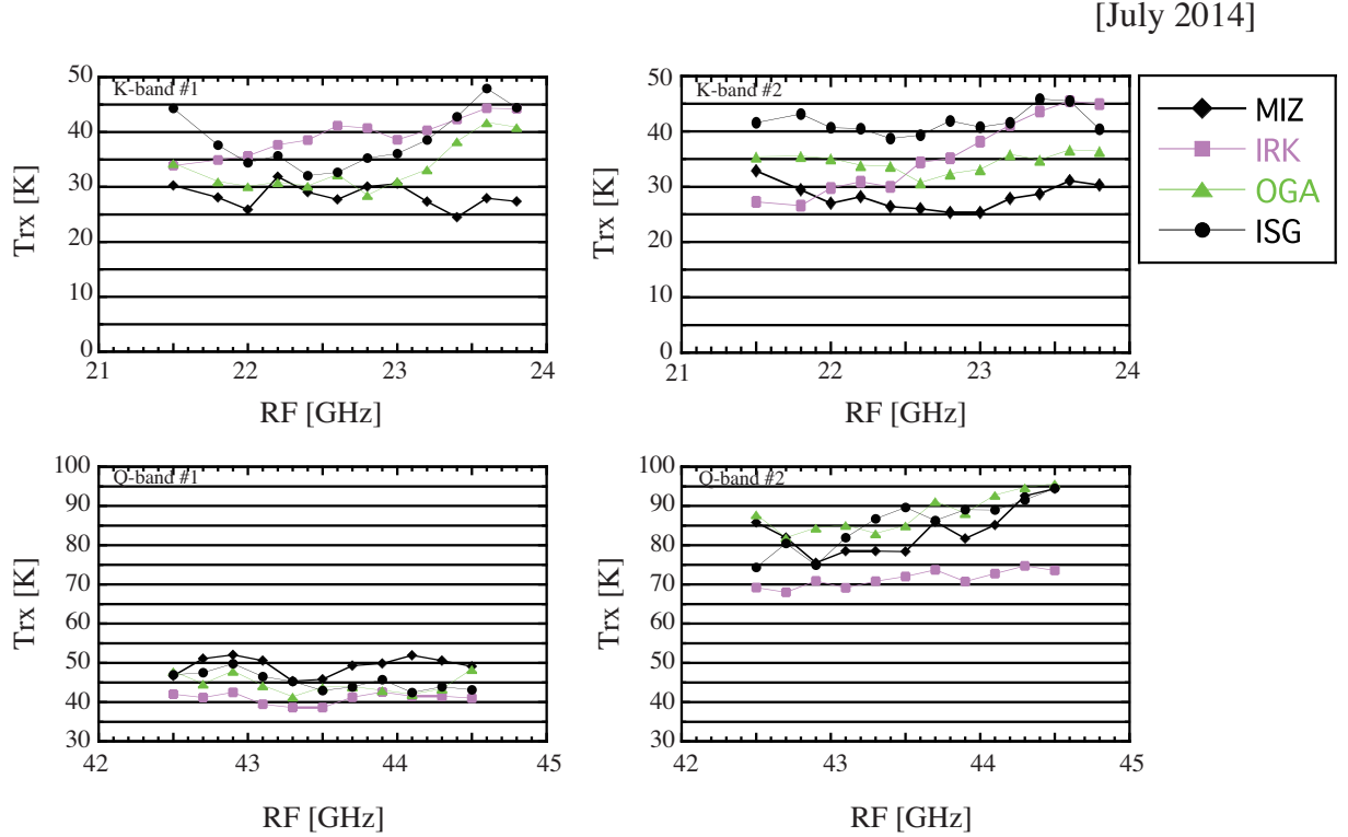
Figure 10: Receiver noise temperature for each VERA antenna. Top and bottom panels show measurements in the K and Q bands, and left and right panels show those in the receiver #1 for beam-A and #2 for beam-B, respectively. Horizontal axis indicate a RF (radio frequency) at which T_{RX} is measured.
