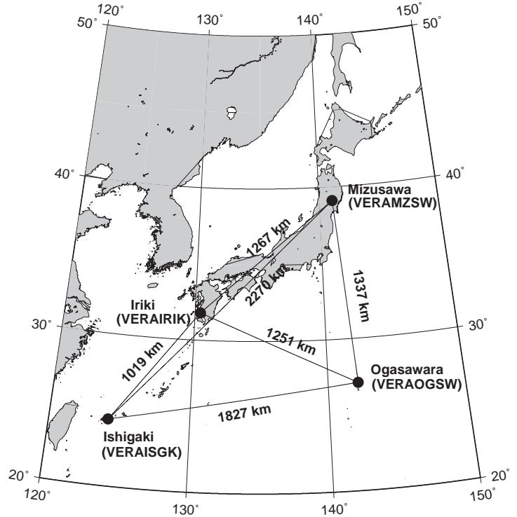
Figure 1: Array configuration of VERA.
