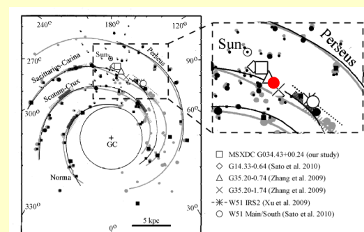
(Sato+ 2010, Kurayama+ 2011)
